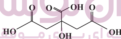
Citric acid
